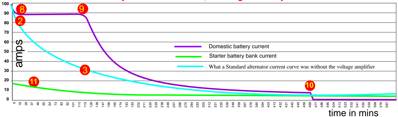
Domestic battery bank current curve, with engine battery bank current curve
